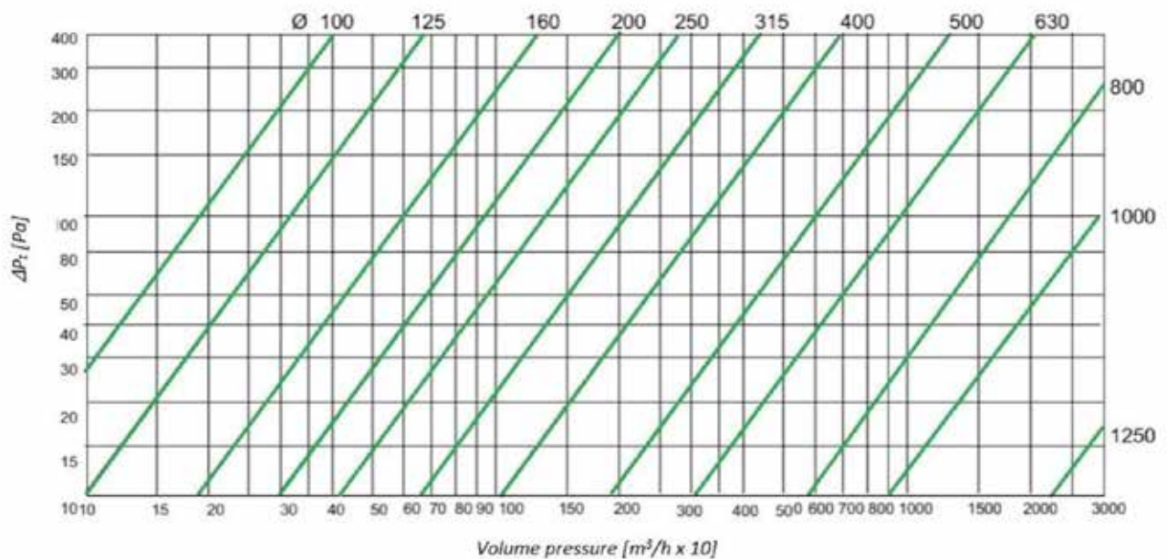
Diagram of pressure loss
